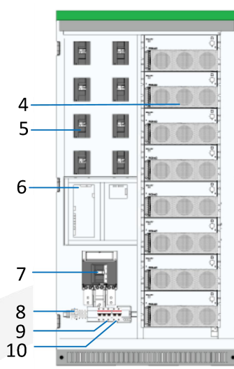
4/8 Strings Version
